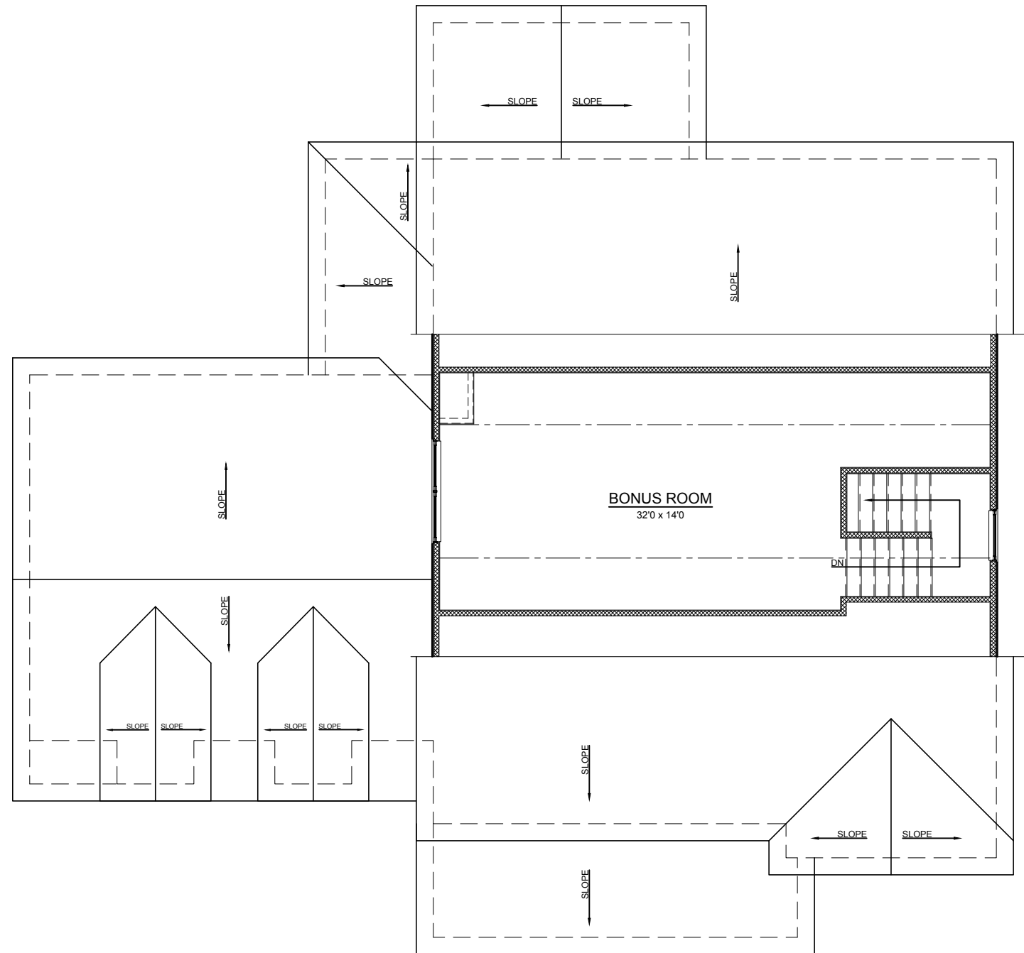
BONUS LEVEL PLAN OLIVE TRACT HOUSE
